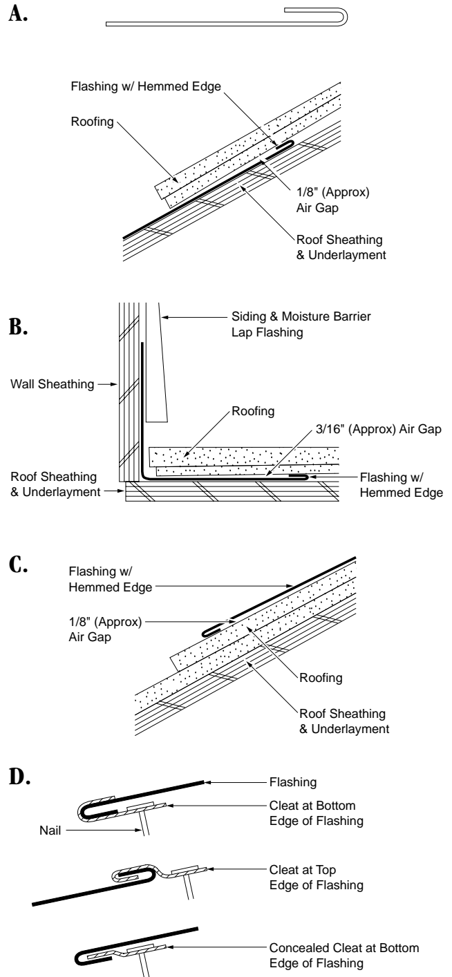
Figure 6-27: The hemmed edge is a very important detail for roof flashing.
