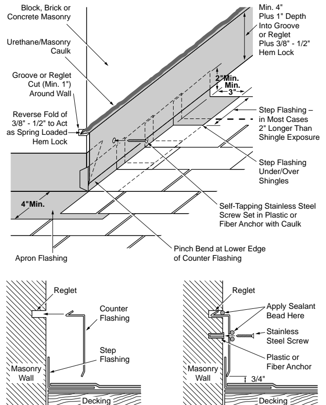
Figure 6-14: Continuous counter flashing against masonry chimneys and walls.
