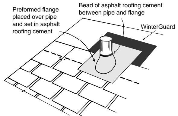
Figure 6-6: Placement of flange over vent pipe.
