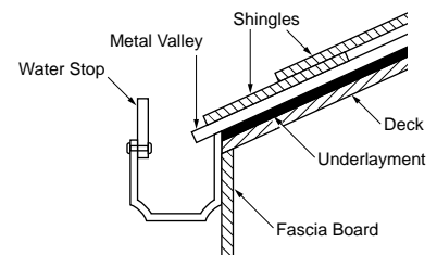
Figure 6-28: Valley side view
