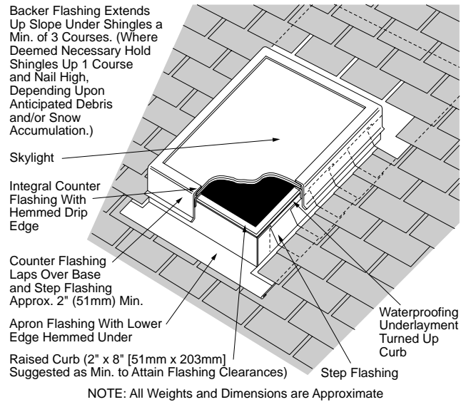
Figure 6-26: Basic sheet metal components used at skylight.
